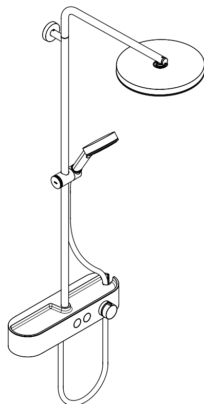
Showerpipe 260 1jet
